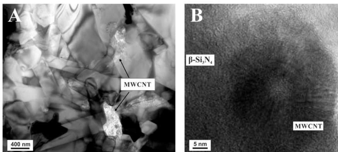
Figure 1. Structural study of Si 3 N 4 /MWCNT substrate: A) TEM image of sintered composite, B) HREM detail of MWCNT and Si 3 N 4 grain boundary
