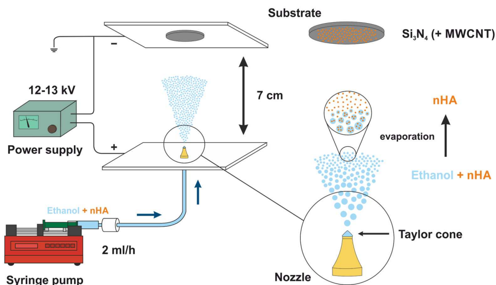
Figure 3. Schematic diagram of the electrospray deposition set-up
